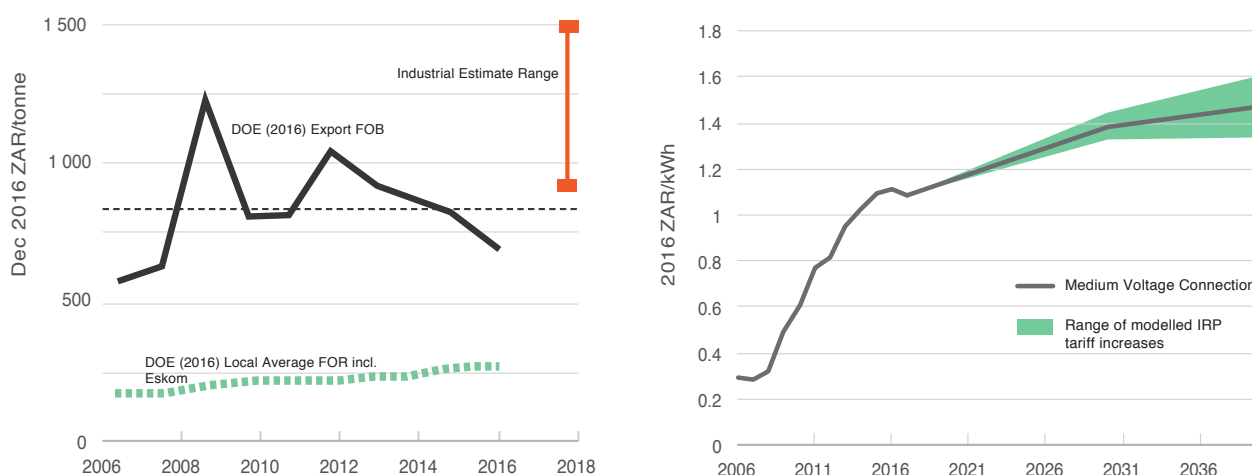
FIGURE 5: (a) Historical local and export coal prices (b) Historical and projected electricity prices
