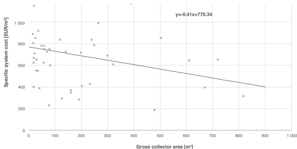
FIGURE 12: Estimated system costs
