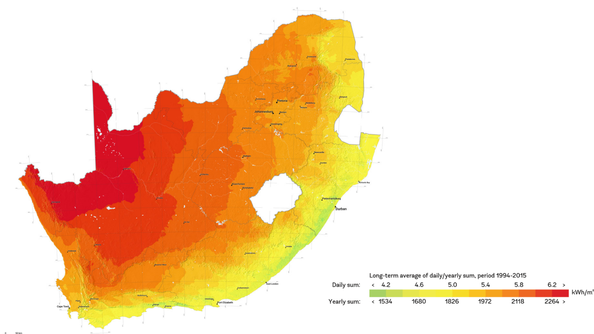
FIGURE 8A: Annual Global Horizontal Irradiation (GHI)
