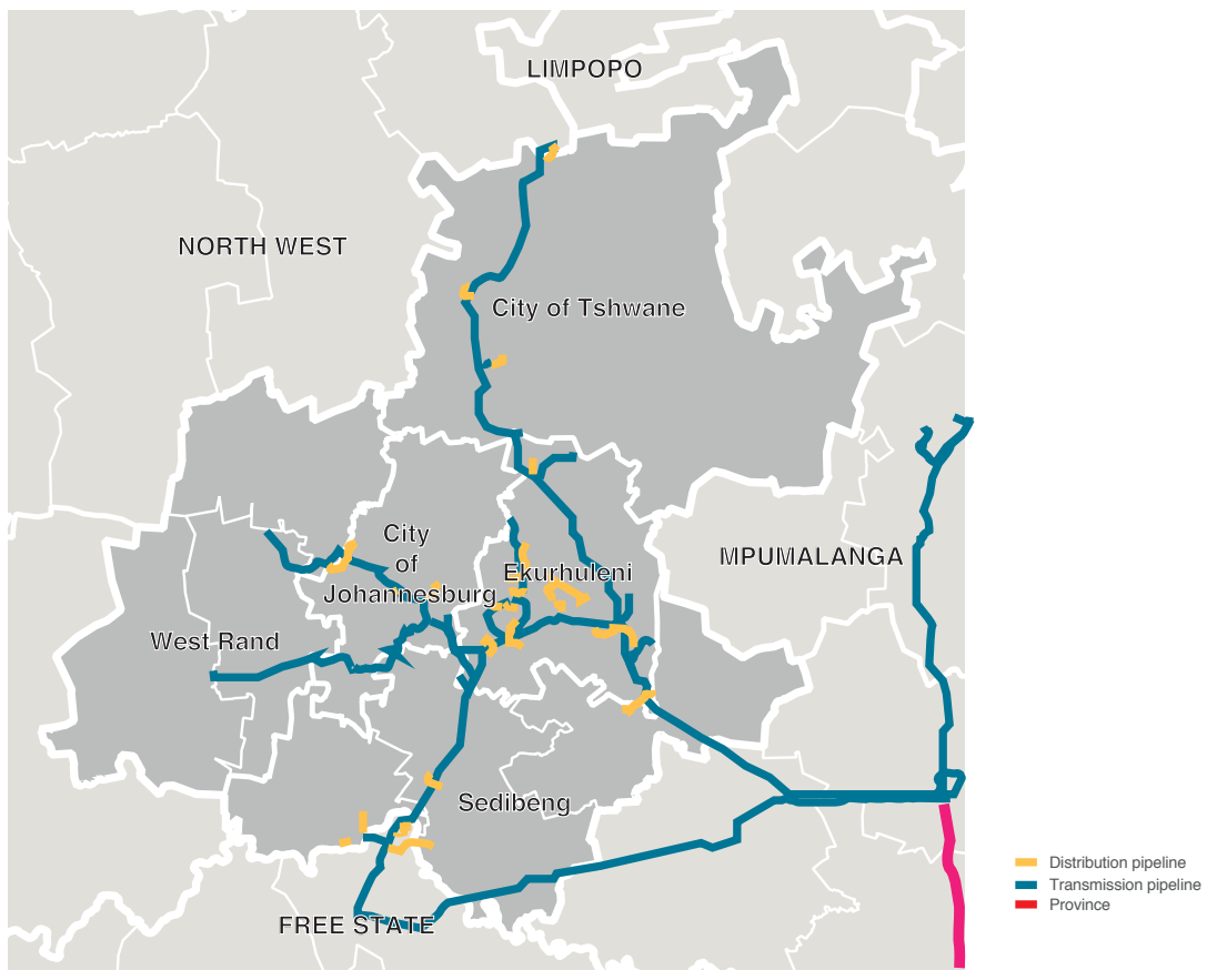
FIGURE 7b: Gas reticulation network in Gauteng (owned by Egoli Gas)
