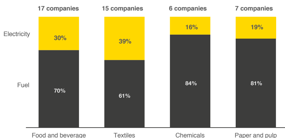
FIGURE 17: Comparison of fuel and electricity consumption in some companies from NCPC audit data
